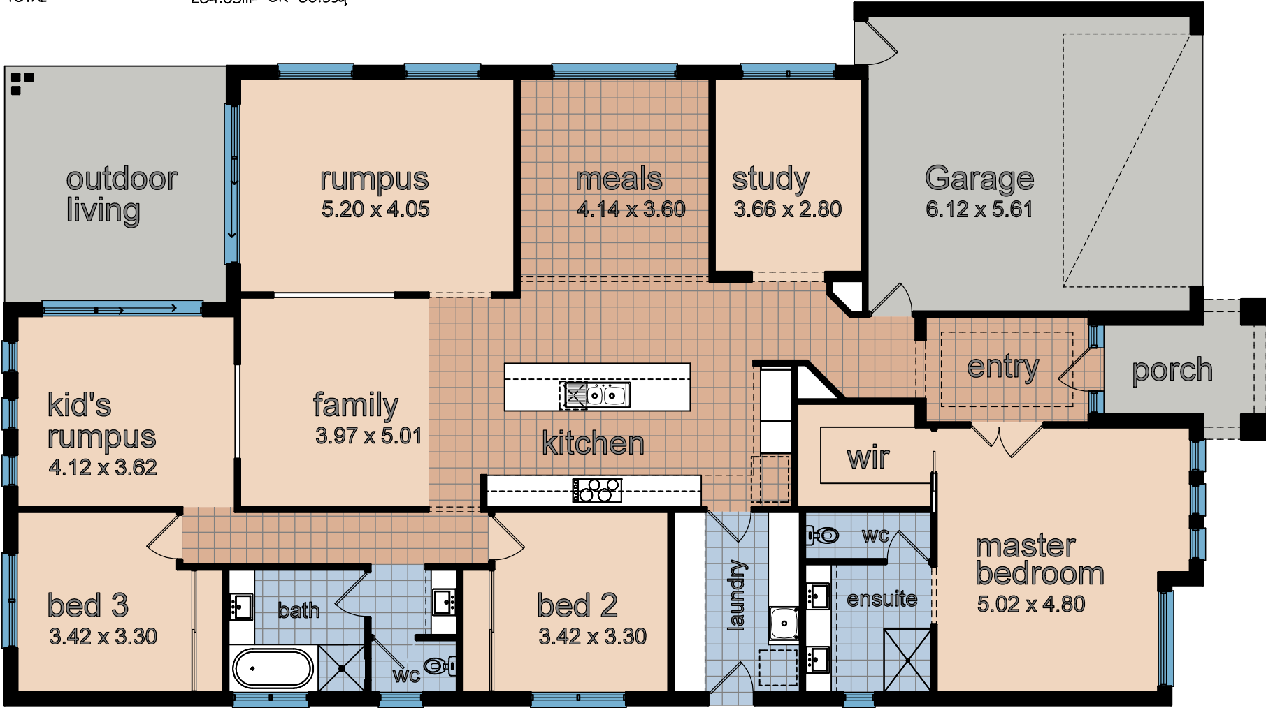
ASPEN FLOOR PLAN
